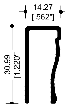
9525 MARCO 1 \frac{1}{4} "
