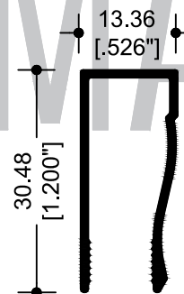
13563 MARCO 1 \frac{1}{4} "
