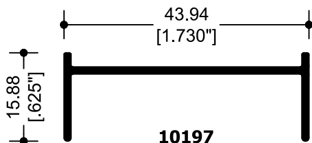
10197 JAMBA LATERAL
