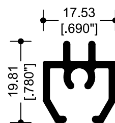
63727 BARROTILLO 2"
