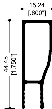
9756 MARCO 1 \frac{3}{4} "
